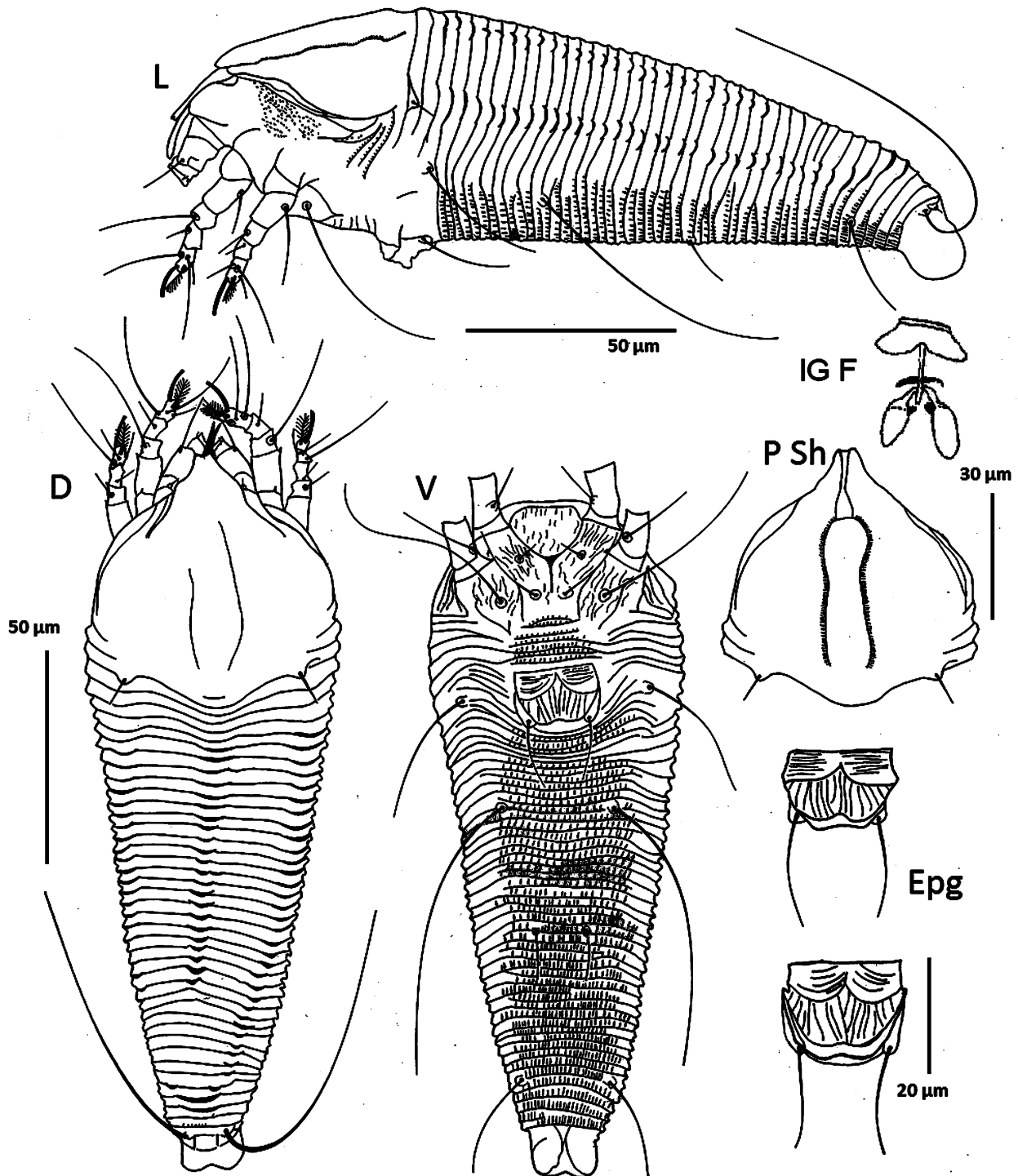
FIGURE 1. Abacarus doctus n. sp. L. Lateral habitus of female; D. Dorsal habitus of female; V. Ventral habitus of female. P Sh. Prodorsal shield ornamentation in detail; Epg. Epigynum, IG F. Internal genitalia of female.
