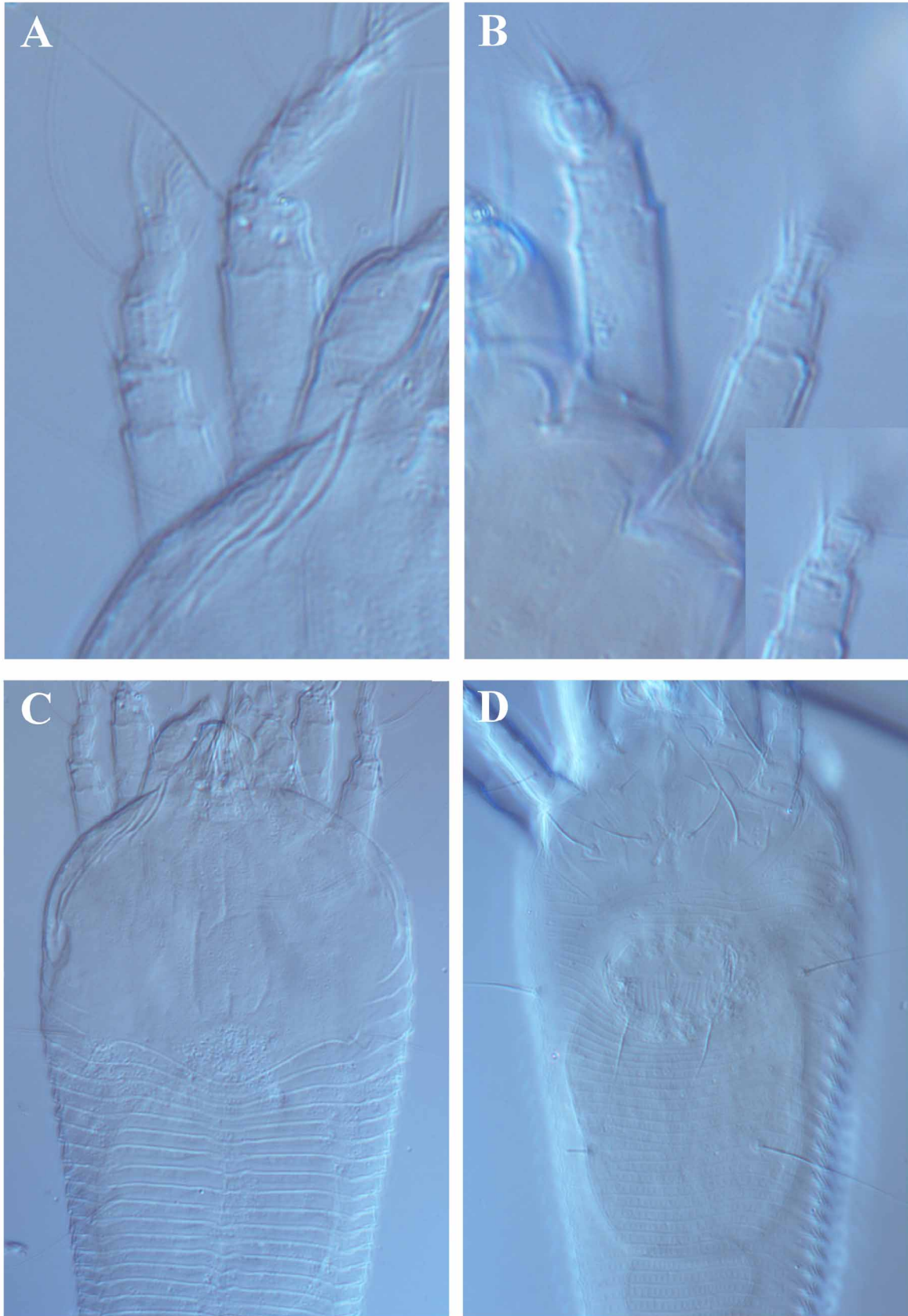
FIGURE 3. Abacarus doctus n. sp. Micrographs showing: A. and B. Tibial seta ( l' ) on dorsal position of Leg II; C. Prodorsal shield; D. Coxigenital region. The specimen in the micrograph appears to show an incomplete median line on the prodorsal shield. However, such a line was not visible on any of the specimens studied under phase contrast or DIC microscopy.
